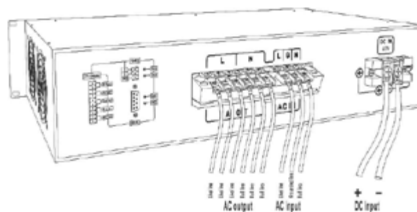
Connecting Cable
